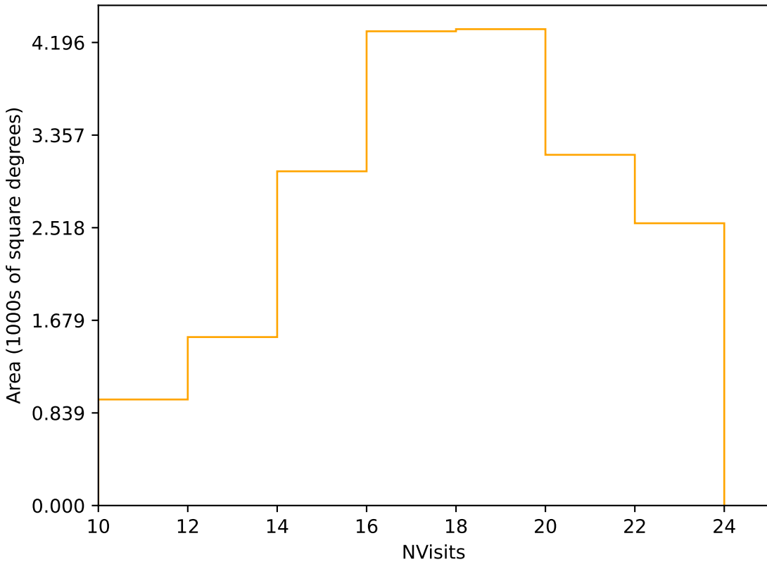
roll_pause_mjdp365_v3.4_10yrs Yr 1 r band: NVisits
