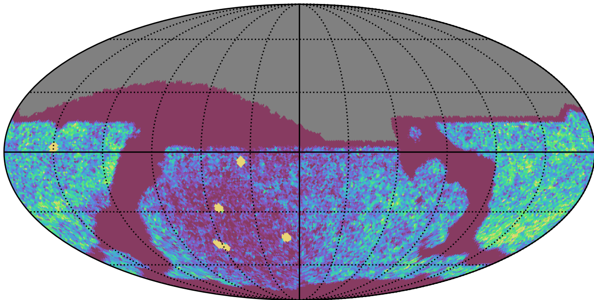
roll_pause_mjdp365_v3.4_10yrs Yr 1 all bands: NVisits
