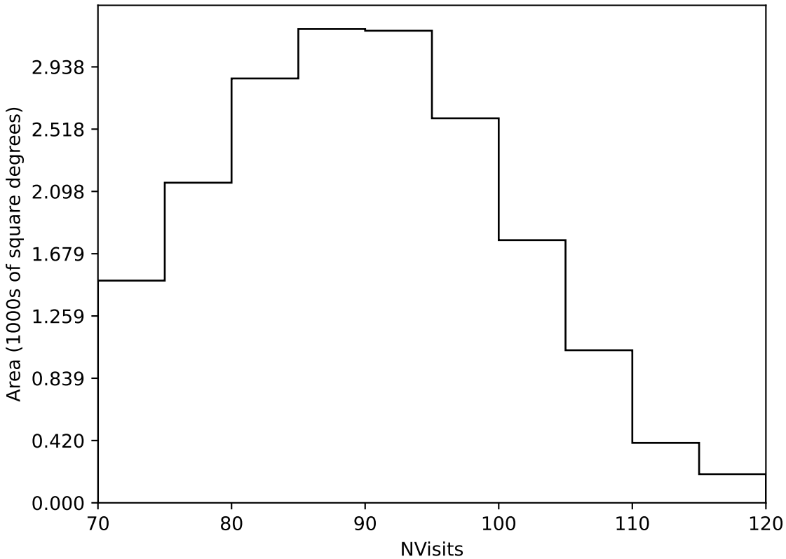
roll_pause_mjdp365_v3.4_10yrs Yr 1 all bands: NVisits
