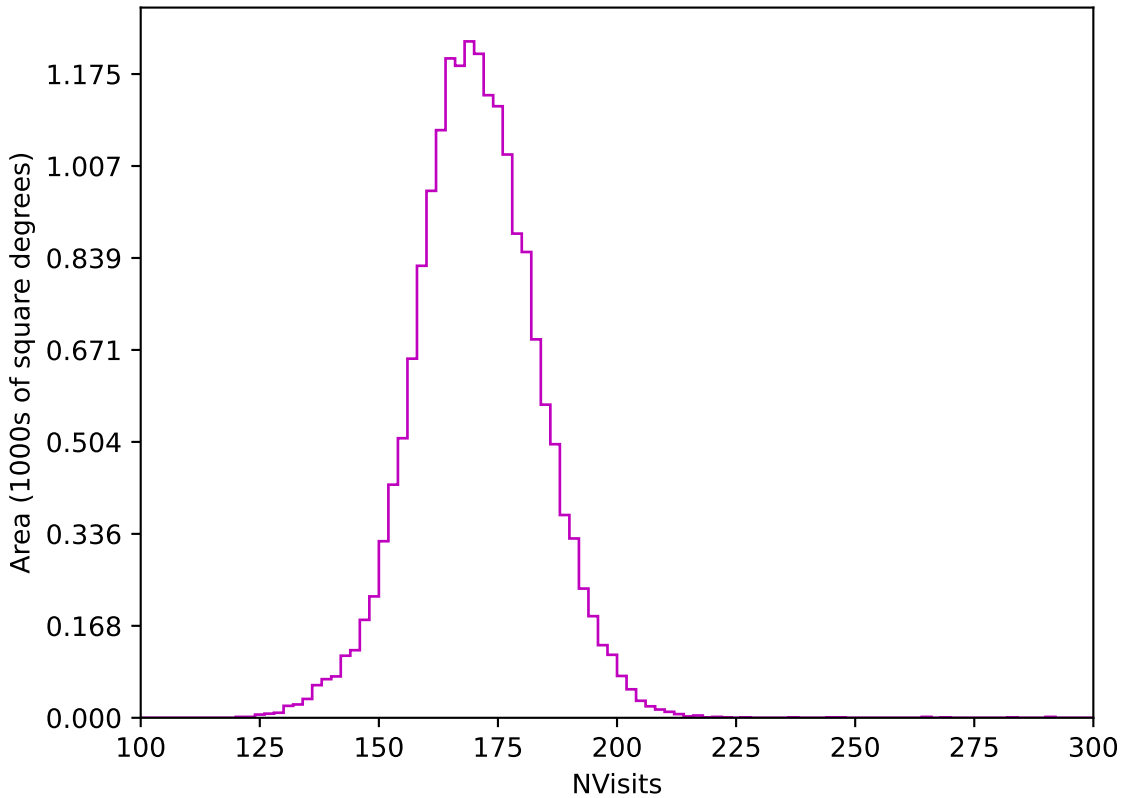
roll_pause_mjdp365_v3.4_10yrs WFD z band: NVisits
