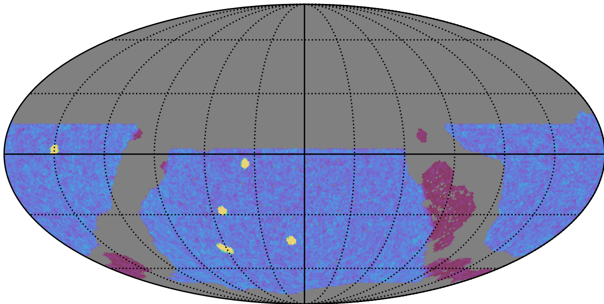
roll_pause_mjdp365_v3.4_10yrs WFD y band: NVisits
