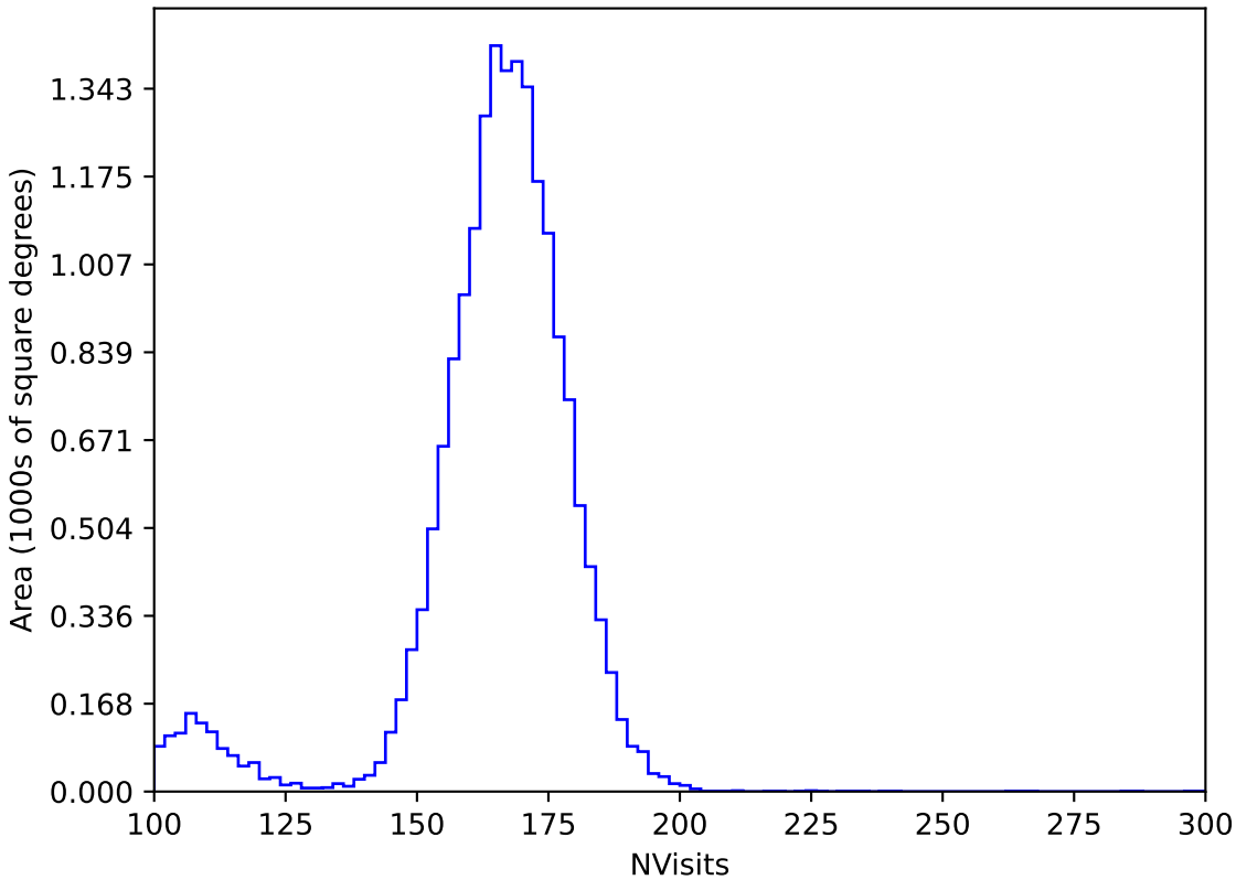
roll_pause_mjdp365_v3.4_10yrs WFD y band: NVisits
