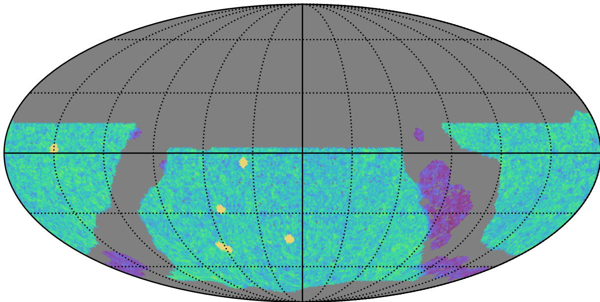
roll_pause_mjdp365_v3.4_10yrs WFD u band: NVisits
