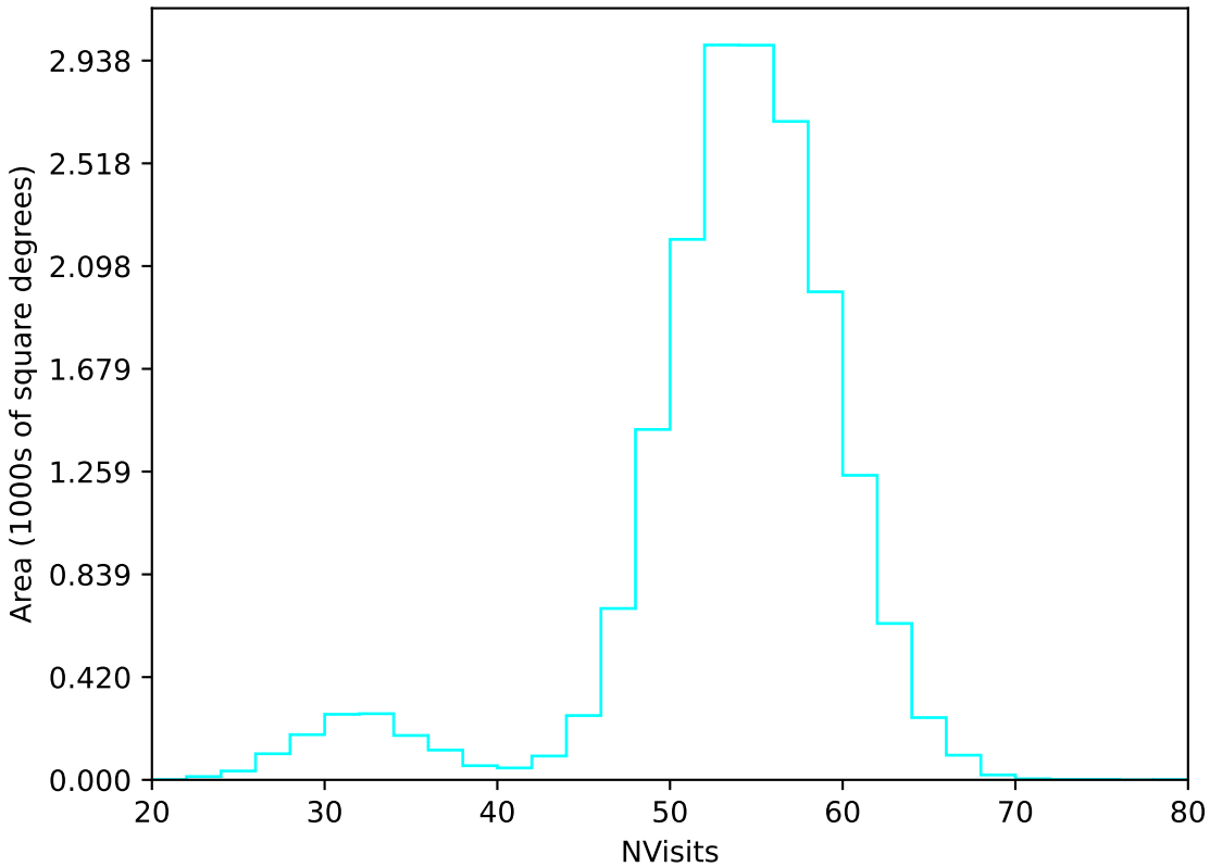
roll_pause_mjdp365_v3.4_10yrs WFD u band: NVisits
