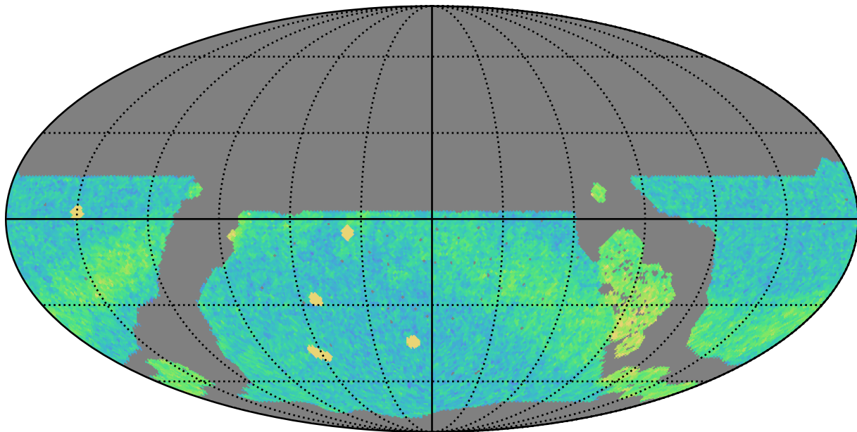
roll_pause_mjdp365_v3.4_10yrs WFD r band: NVisits
