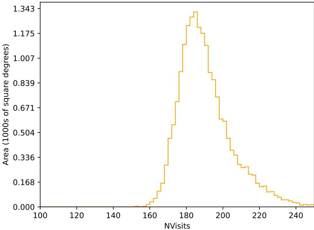
roll_pause_mjdp365_v3.4_10yrs WFD r band: NVisits
