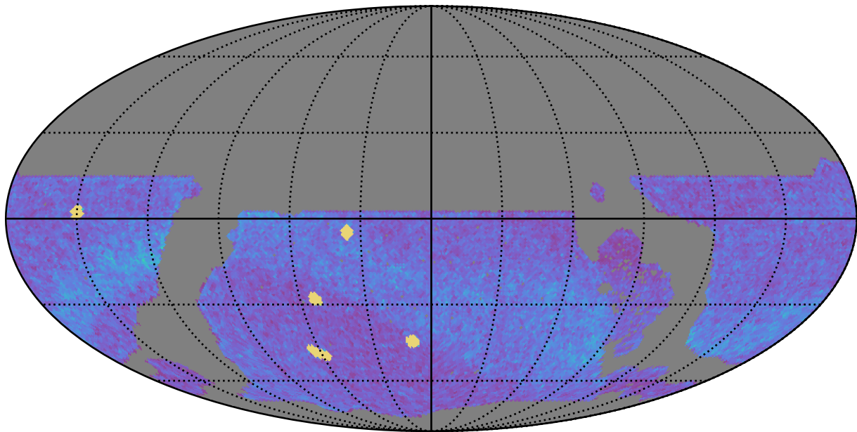
roll_pause_mjdp365_v3.4_10yrs WFD all bands: NVisits
