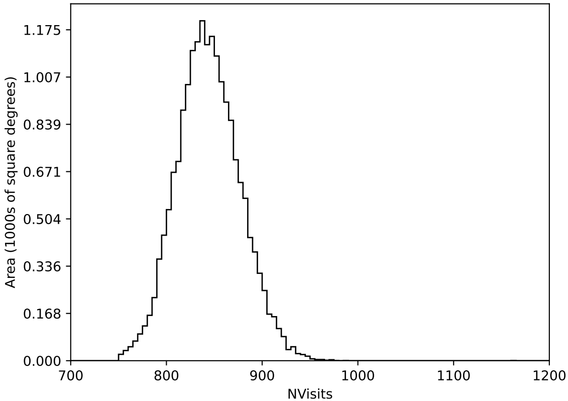
roll_pause_mjdp365_v3.4_10yrs WFD all bands: NVisits
