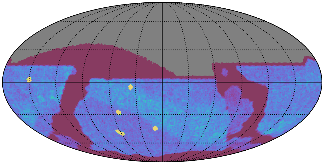
roll_pause_mjdp365_v3.4_10yrs All sky z band: NVisits
