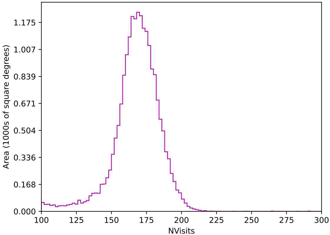
roll_pause_mjdp365_v3.4_10yrs All sky z band: NVisits
