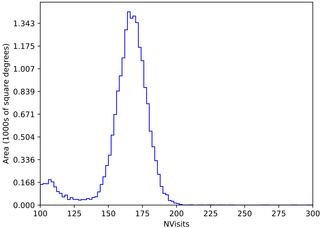
roll_pause_mjdp365_v3.4_10yrs All sky y band: NVisits
