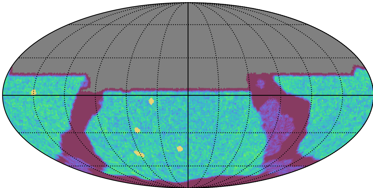
roll_pause_mjdp365_v3.4_10yrs All sky u band: NVisits
