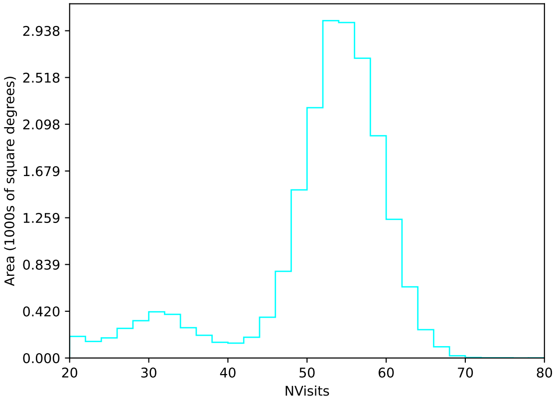
roll_pause_mjdp365_v3.4_10yrs All sky u band: NVisits
