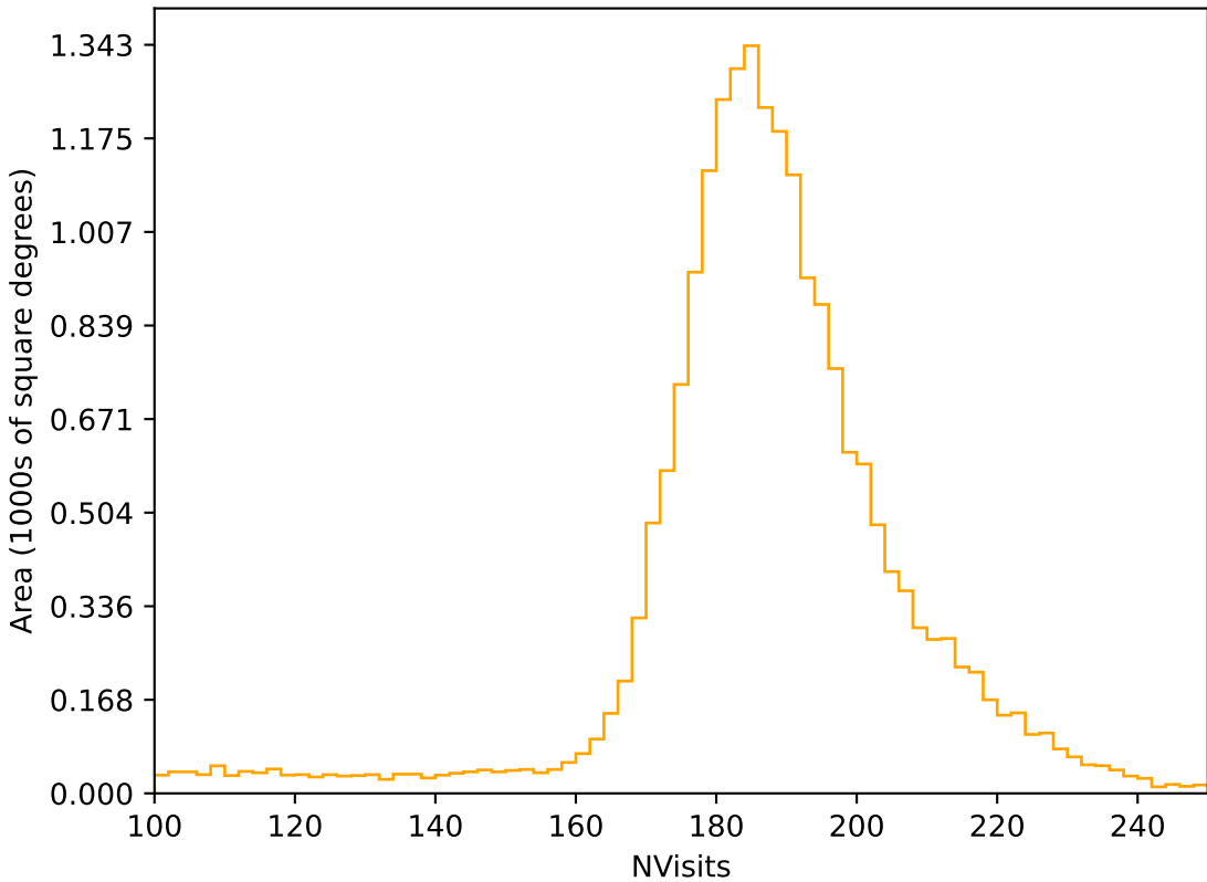
roll_pause_mjdp365_v3.4_10yrs All sky r band: NVisits
