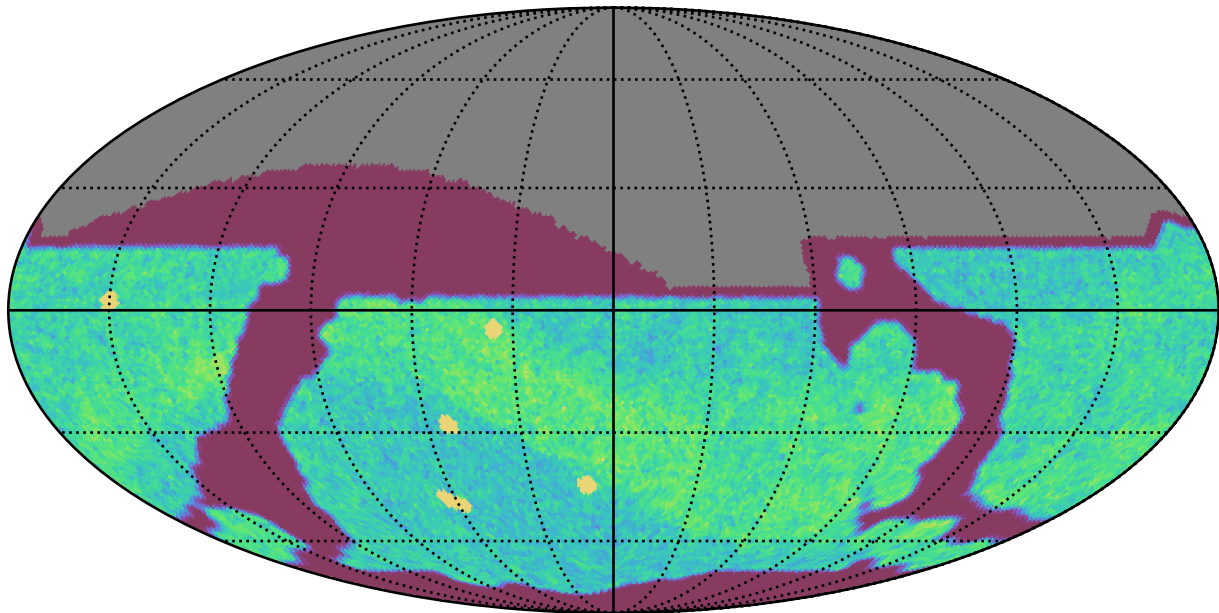
roll_pause_mjdp365_v3.4_10yrs All sky i band: NVisits
