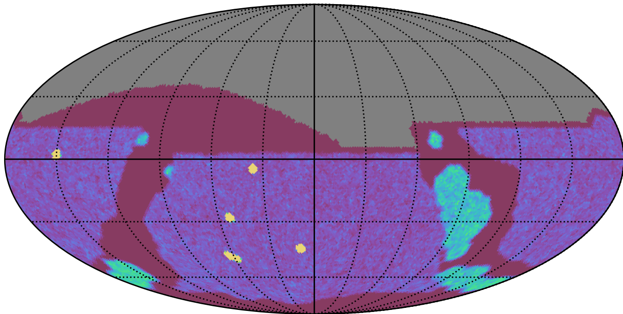
roll_pause_mjdp365_v3.4_10yrs All sky g band: NVisits
