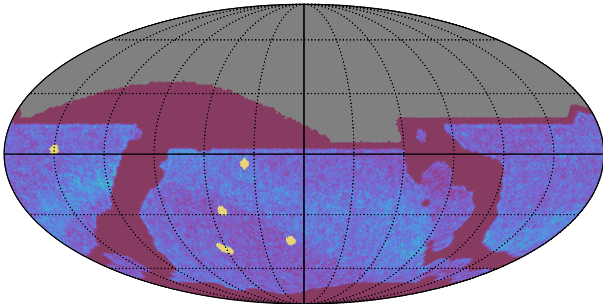
roll_pause_mjdp365_v3.4_10yrs All sky all bands: NVisits
