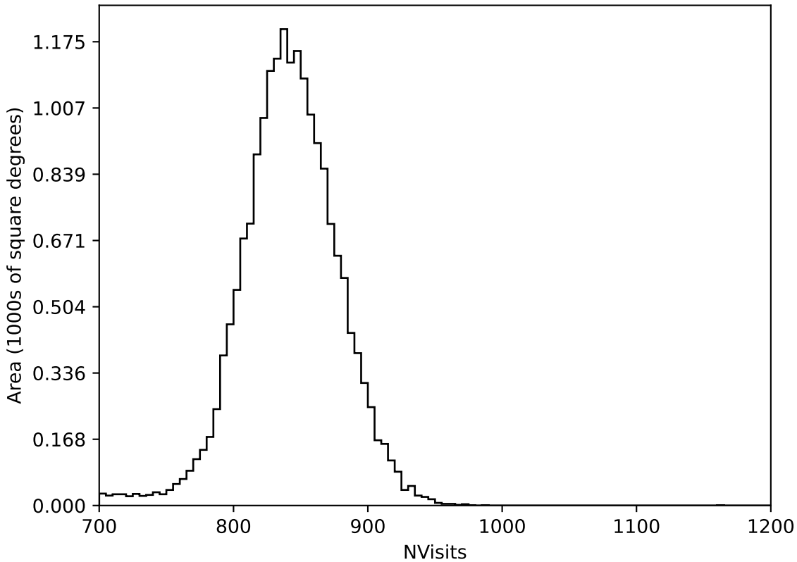
roll_pause_mjdp365_v3.4_10yrs All sky all bands: NVisits
