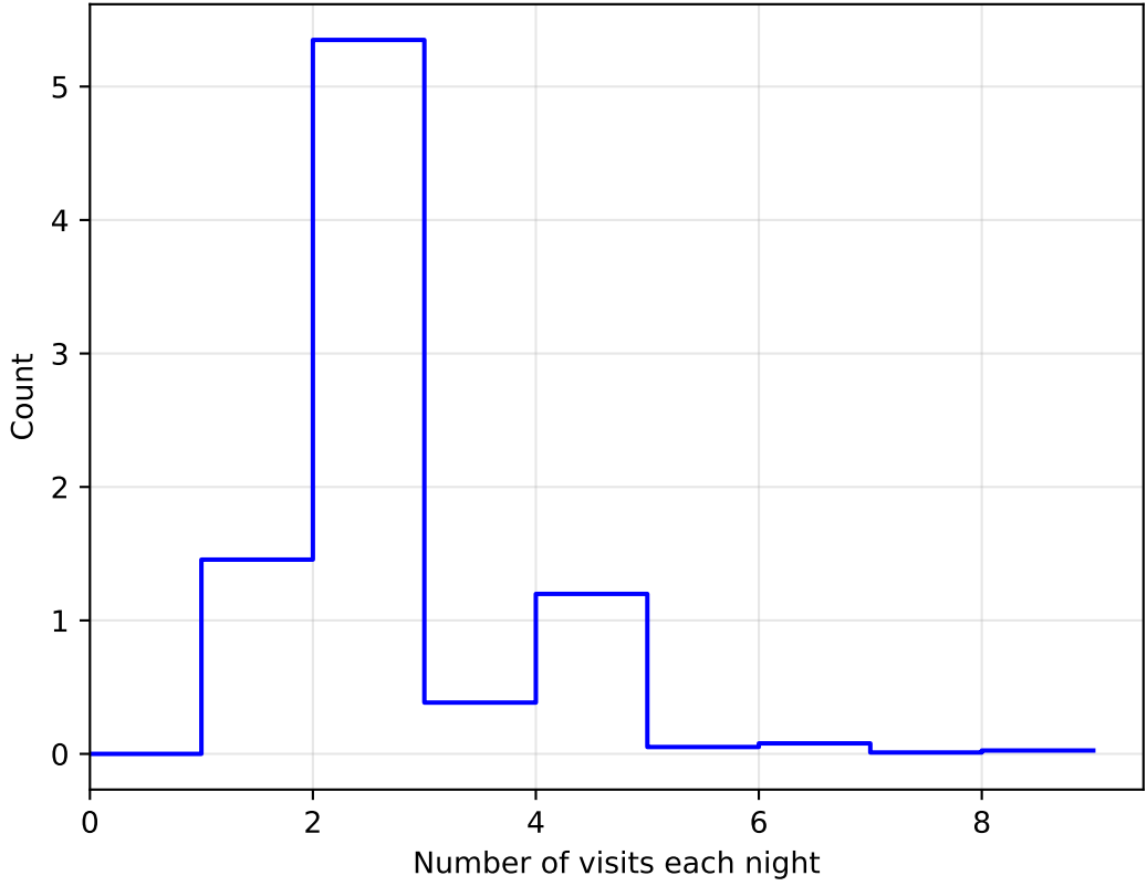
roll_pause_mjdp365_v3.4_10yrs WFD: NVisitsPerNight
