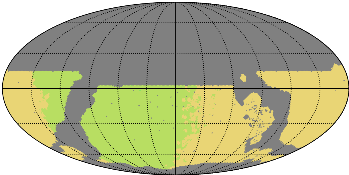
roll_pause_mjdp365_v3.4_10yrs WFD all bands: NSeasons
