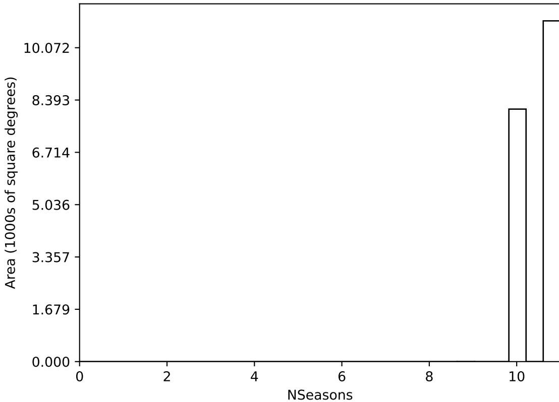
roll_pause_mjdp365_v3.4_10yrs WFD all bands: NSeasons
