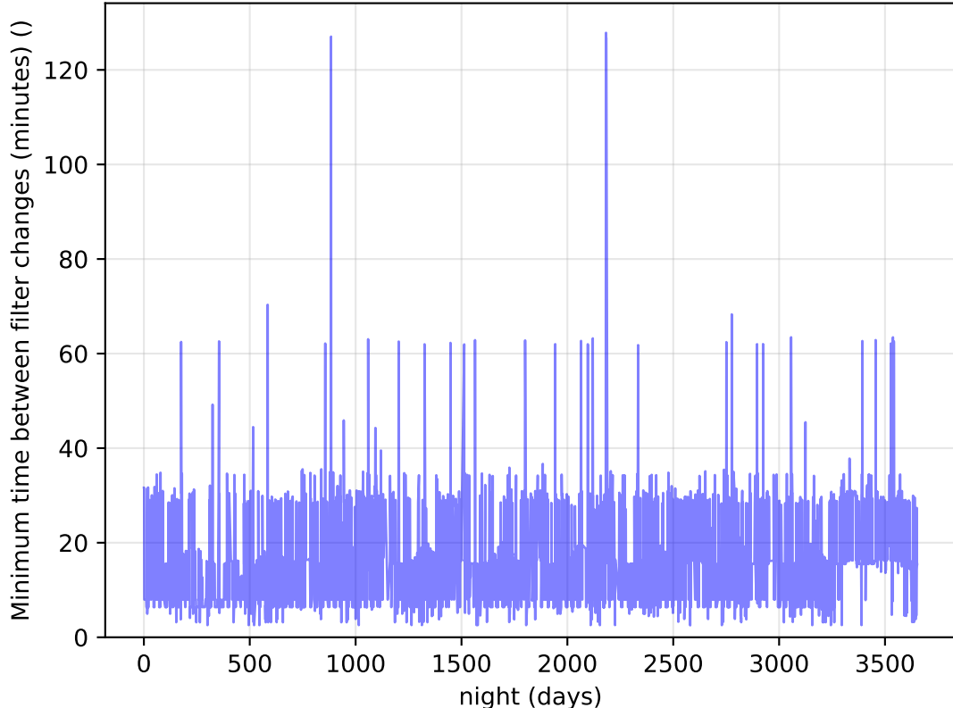
roll_pause_mjdp365_v3.4_10yrs Per Night: Minimum time between filter changes (minutes)
