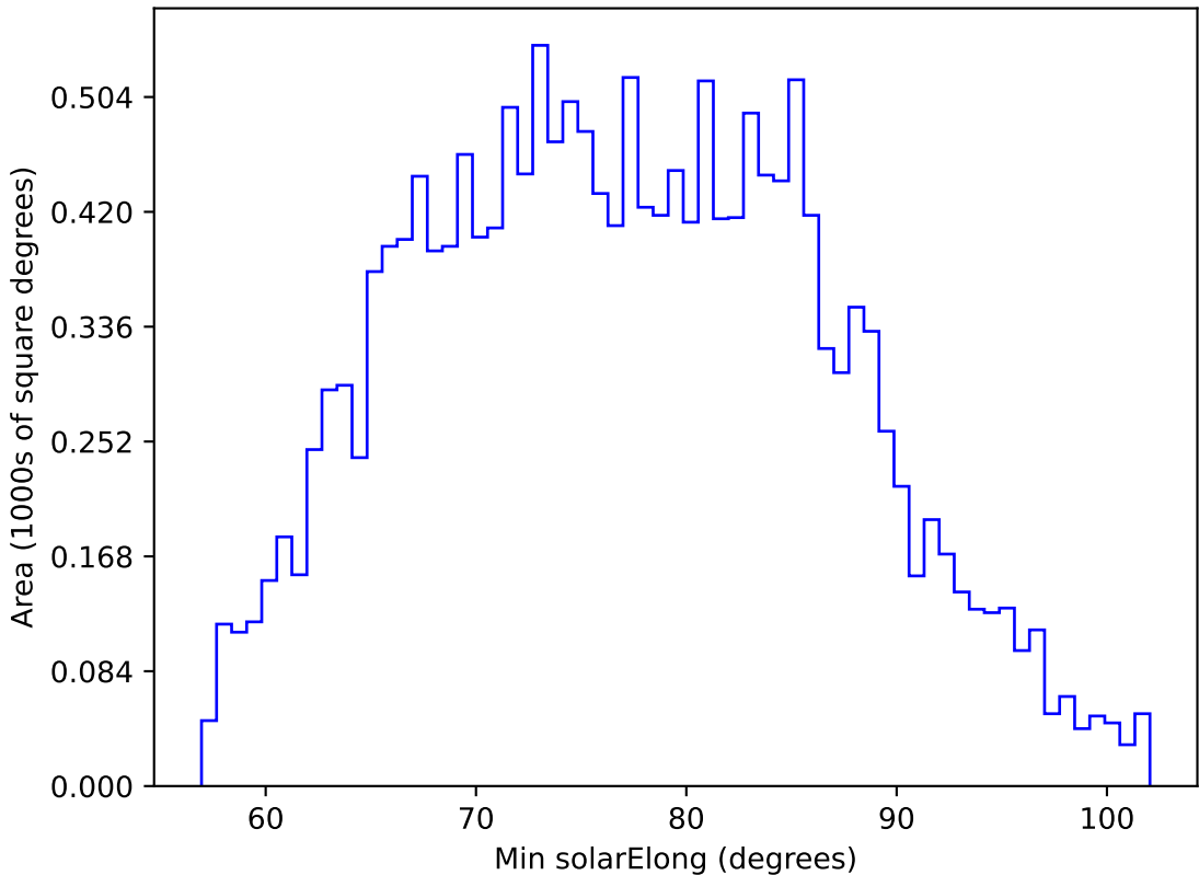
roll_pause_mjdp365_v3.4_10yrs WFD u band: Min solarElong
