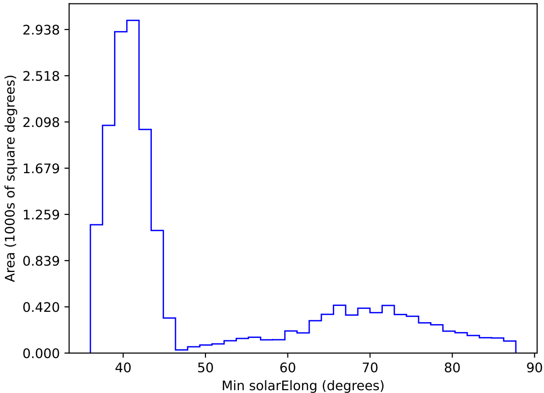
roll_pause_mjdp365_v3.4_10yrs WFD i band: Min solarElong
