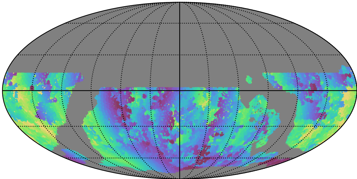
roll_pause_mjdp365_v3.4_10yrs WFD g band: Min solarElong
