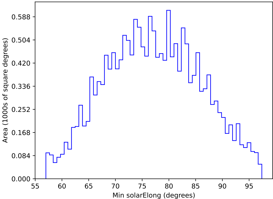
roll_pause_mjdp365_v3.4_10yrs WFD g band: Min solarElong
