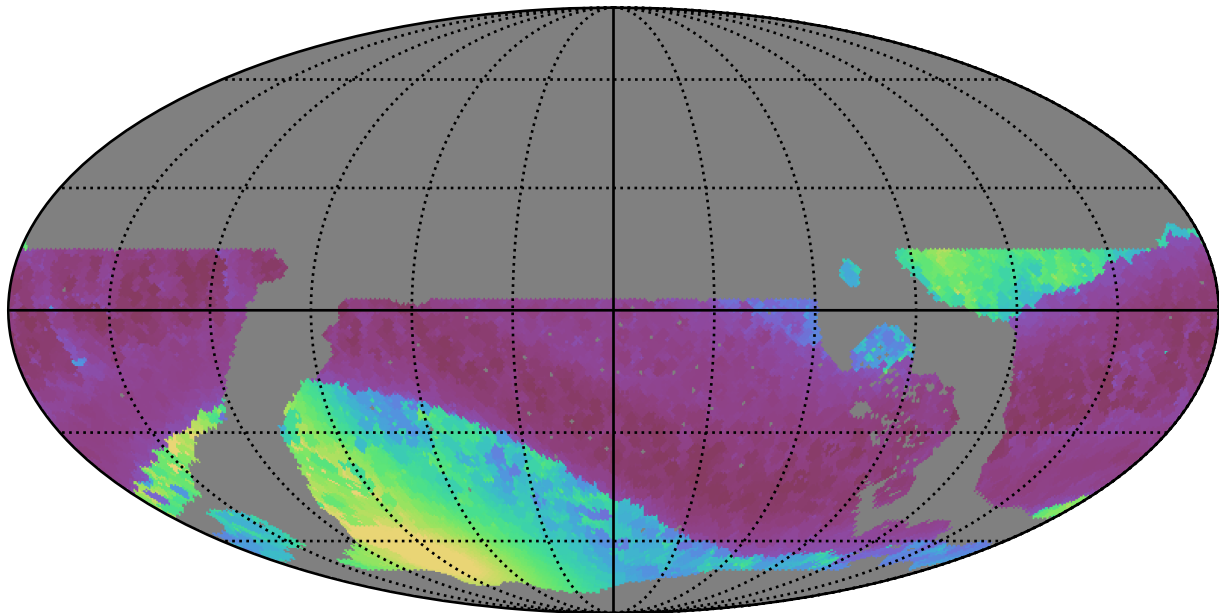
roll_pause_mjdp365_v3.4_10yrs WFD all bands: Min solarElong
