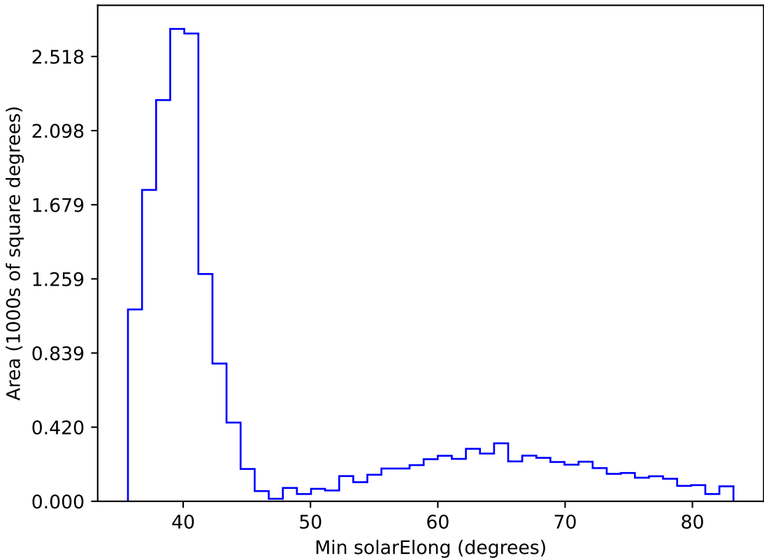
roll_pause_mjdp365_v3.4_10yrs WFD all bands: Min solarElong
