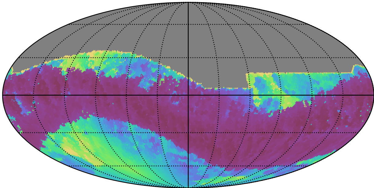
roll_pause_mjdp365_v3.4_10yrs All sky z band: Min solarElong
