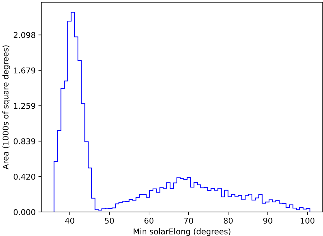
roll_pause_mjdp365_v3.4_10yrs All sky z band: Min solarElong
