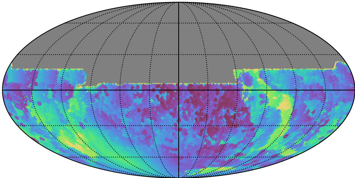
roll_pause_mjdp365_v3.4_10yrs All sky y band: Min solarElong
