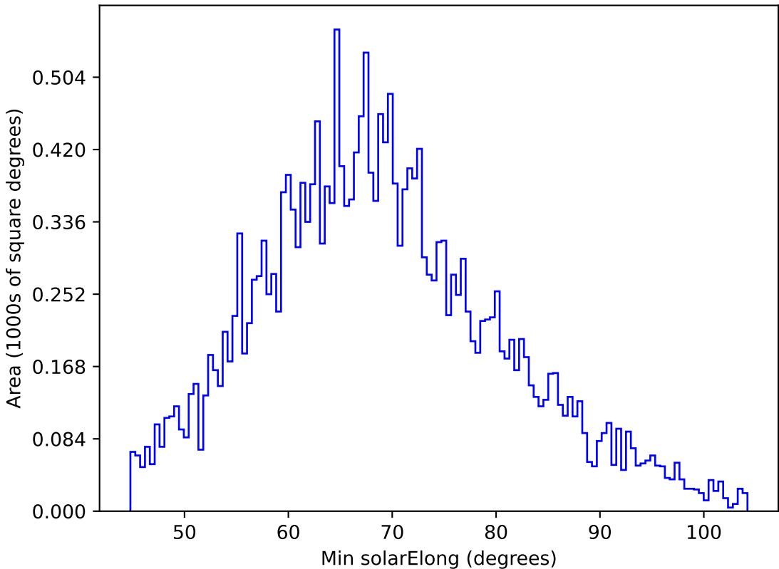
roll_pause_mjdp365_v3.4_10yrs All sky y band: Min solarElong
