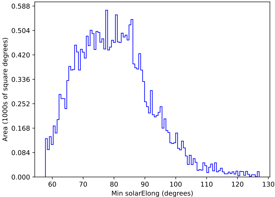
roll_pause_mjdp365_v3.4_10yrs All sky u band: Min solarElong
