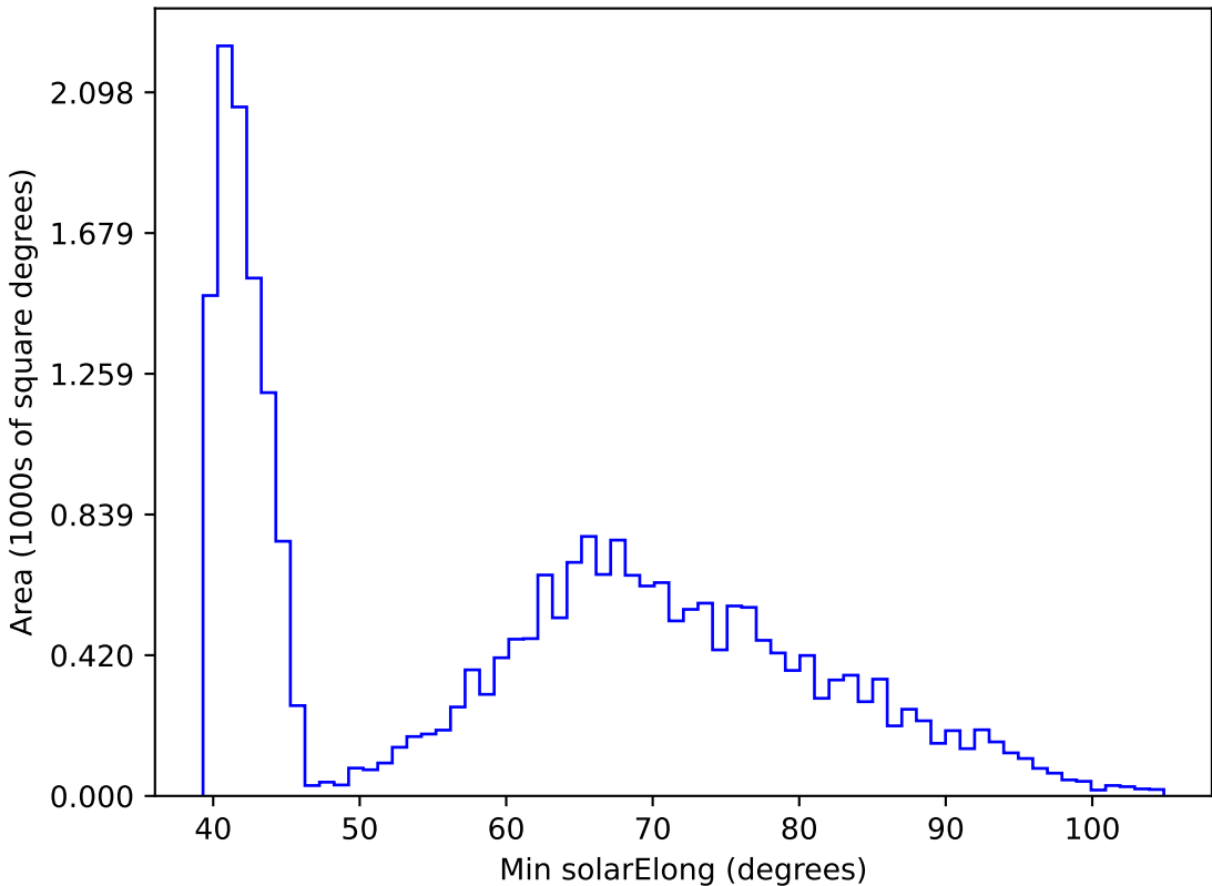
roll_pause_mjdp365_v3.4_10yrs All sky r band: Min solarElong
