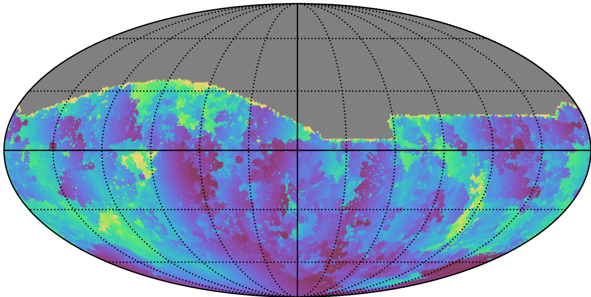
roll_pause_mjdp365_v3.4_10yrs All sky g band: Min solarElong
