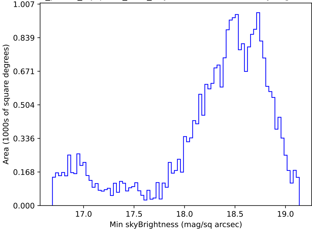
roll_pause_mjdp365_v3.4_10yrs Yr 1 z band: Min skyBrightness
