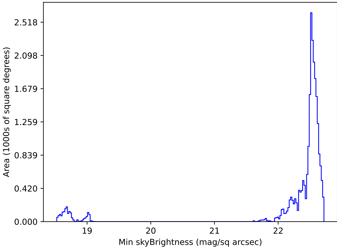
roll_pause_mjdp365_v3.4_10yrs Yr 1 u band: Min skyBrightness
