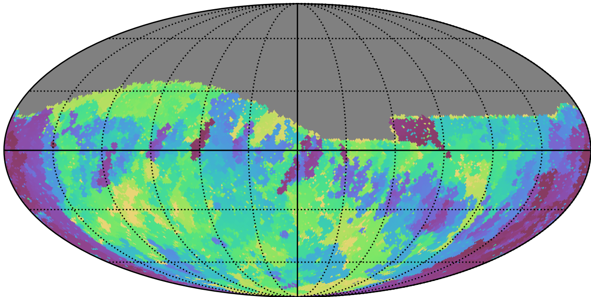
roll_pause_mjdp365_v3.4_10yrs Yr 1 r band: Min skyBrightness
