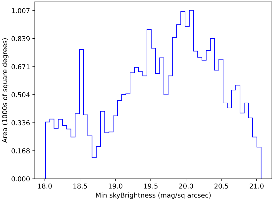
roll_pause_mjdp365_v3.4_10yrs Yr 1 r band: Min skyBrightness
