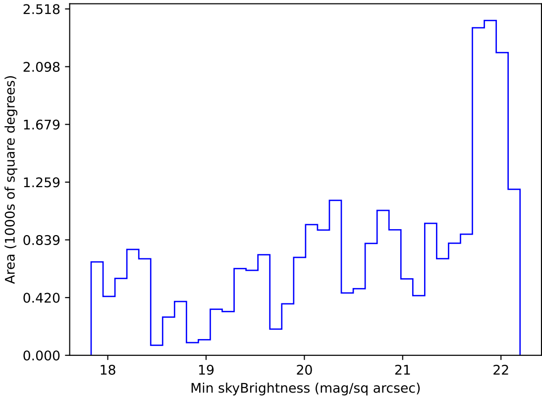
roll_pause_mjdp365_v3.4_10yrs Yr 1 g band: Min skyBrightness
