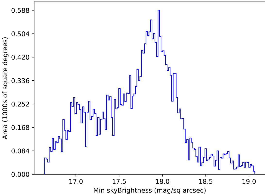
roll_pause_mjdp365_v3.4_10yrs Yr 1 all bands: Min skyBrightness
