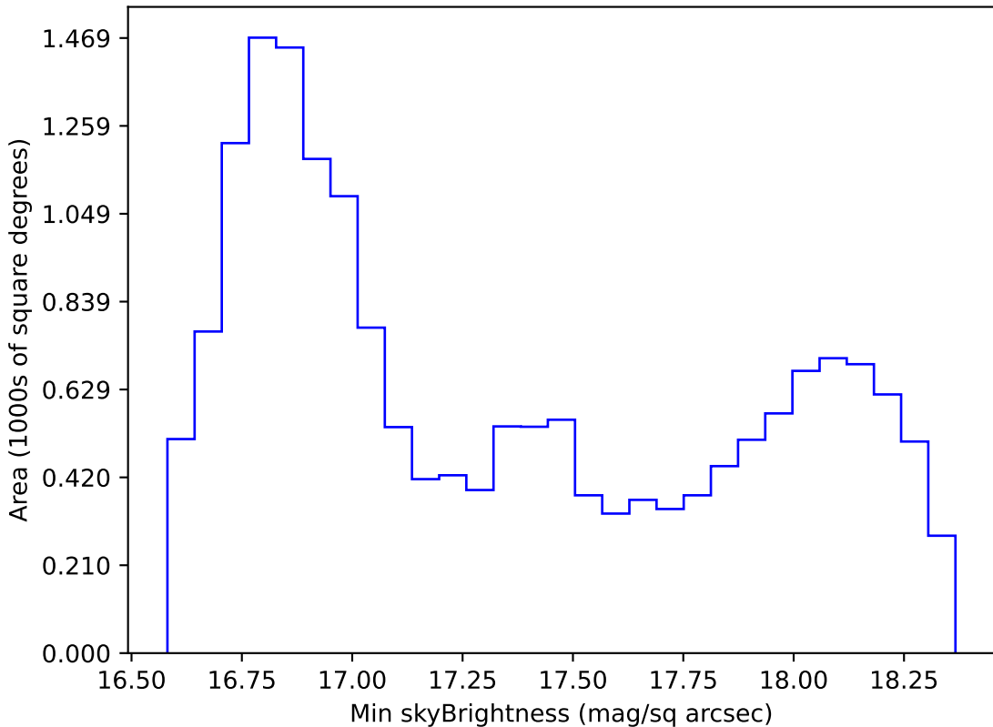
roll_pause_mjdp365_v3.4_10yrs WFD z band: Min skyBrightness
