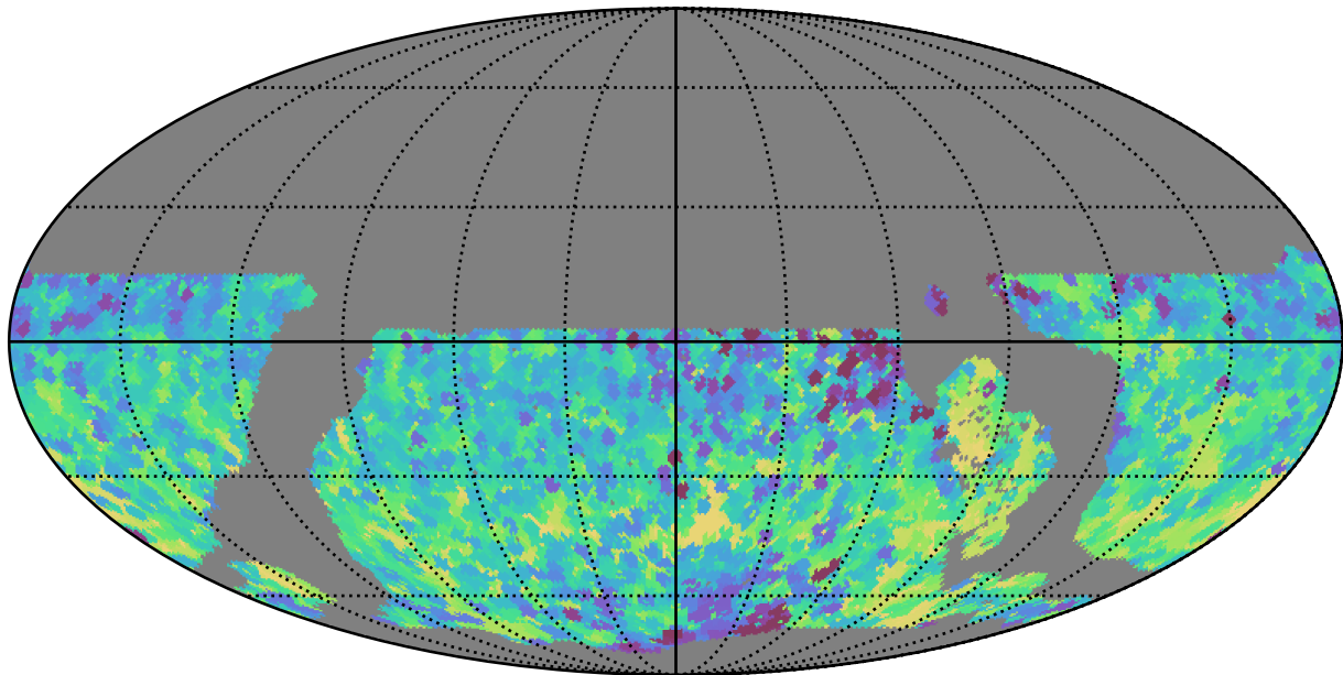
roll_pause_mjdp365_v3.4_10yrs WFD y band: Min skyBrightness
