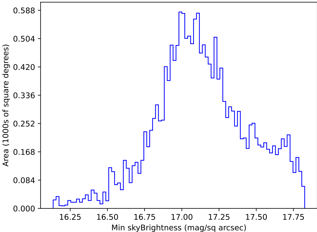
roll_pause_mjdp365_v3.4_10yrs WFD y band: Min skyBrightness
