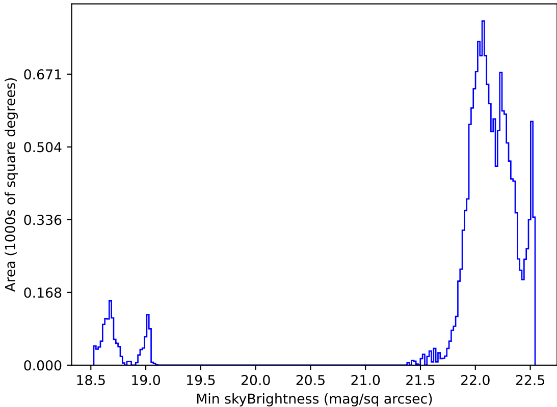
roll_pause_mjdp365_v3.4_10yrs WFD u band: Min skyBrightness
