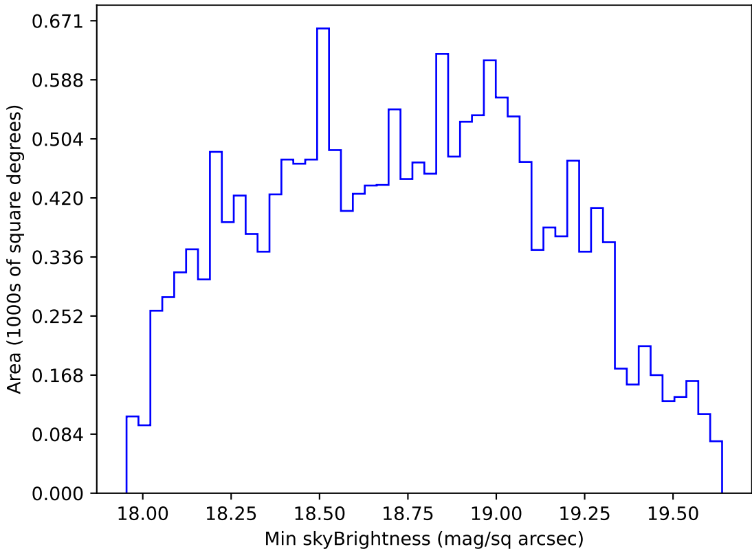
roll_pause_mjdp365_v3.4_10yrs WFD r band: Min skyBrightness
